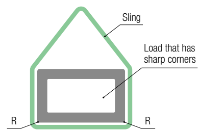
In the case that the sling dimension (H) is greater than the edge radius (R)
